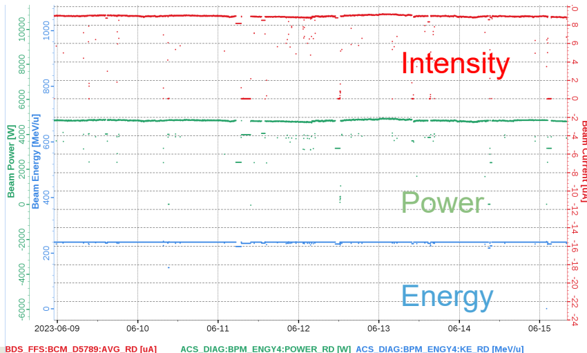
Dual charge state ^{64}\text{Zn}^{28+,29+} for experiment, 150 hrs
