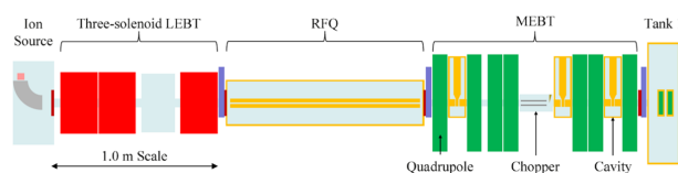
Figure 6: New MEBT to be installed on the ISIS injector.
