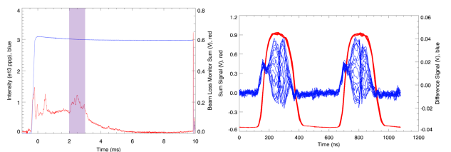
Figure 8: Left: Beam intensity (blue) and sum beam-loss (red) traces as a function of time through the acceleration cycle in RCS operations. The timeframe associated with the beam instability is highlighted. Right: 20-turn extract of the vertical BPM sum (red) and difference (blue) signals during the instability.
