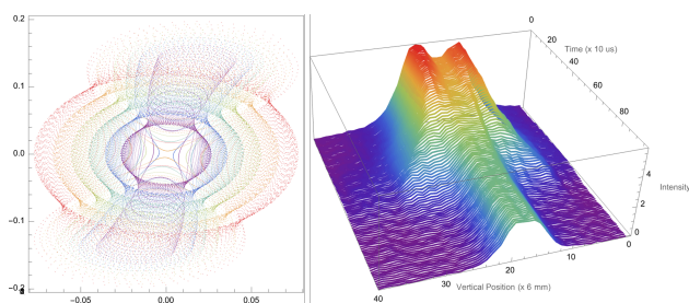
Figure 5: Poincaré map ( y, y' ) during adiabatic crossing of 2Q_y = 7 from simple simulation (left). Measured vertical profile for the beam adiabatically crossing 2Q_y = 7 (right).
