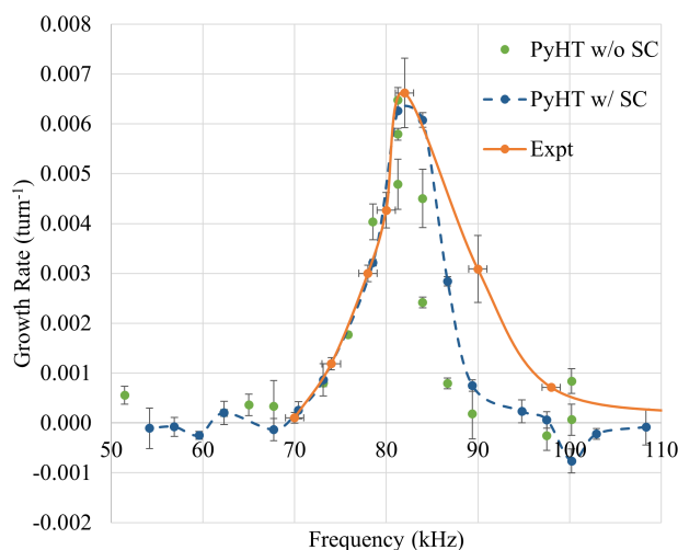
Figure 13: Head-tail instability growth rate versus frequency for experiment (orange) and PyHT simulations with (blue) and without (green) space charge.
