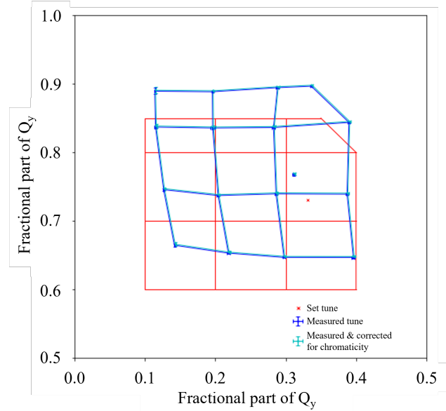
Figure 3: Tune plane showing original linear, “set” tune (red) and measured values (blue).
