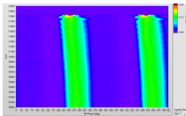
Figure 7: BPM sum signal over the last ~850 turns illustrating bunch compression at extraction from the RCS.
