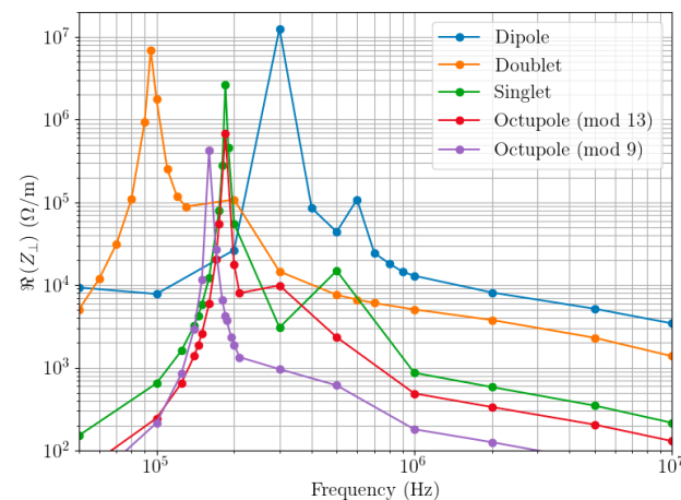
Figure 10: The real part of the transverse impedance for RCS magnet RF screens from CST simulations at low frequency.
